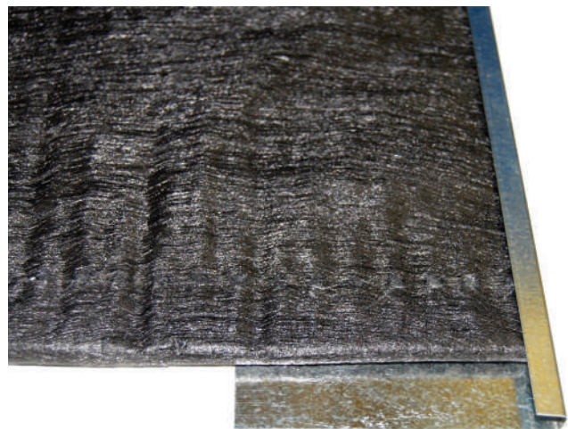
MTI Edge Metal™ accommodates the depth of the Sure Cavity® rainscreen drainage plane
